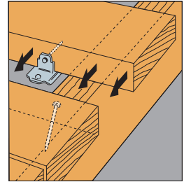
Typical DBT Installation
