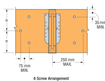
6 Screw Arrangement
