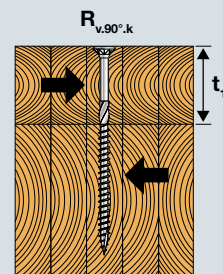
Shear Perpendicular (90°) to the Grain
