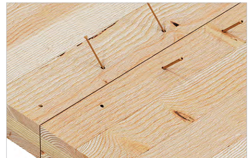
ESCRFTZ screws in installation of CLT butt-joint application.
