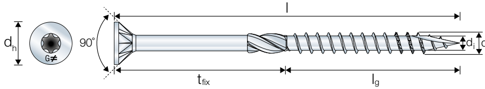
TTSFS - Characteristic Tension and Shear Capacities, Parallel (0°) to the Grain Timber to Timber C24
