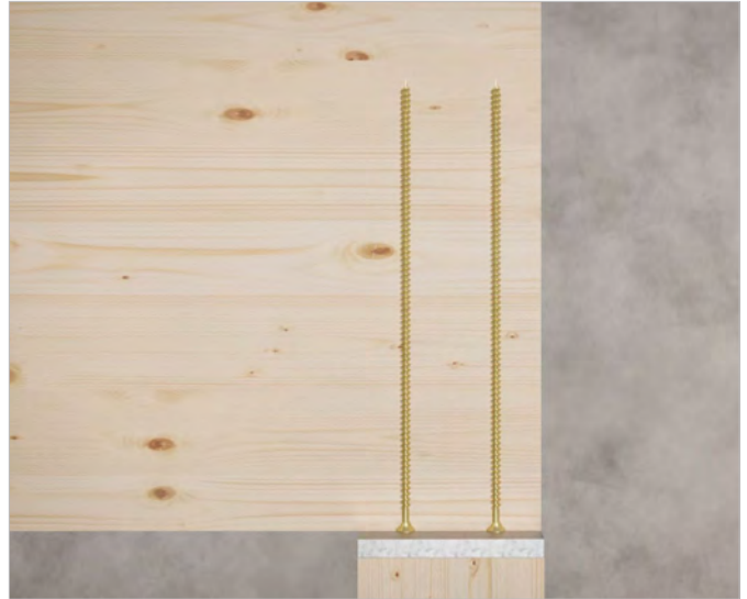
ESCRFTC screws in seat reinforcement application with additional steel plate.
