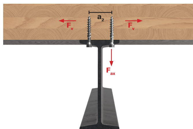
CLT Floor supported above Steel I-Beam
